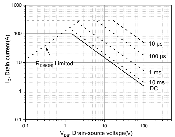
Figure 10. Safe operation area T_C=25^{\circ}C
