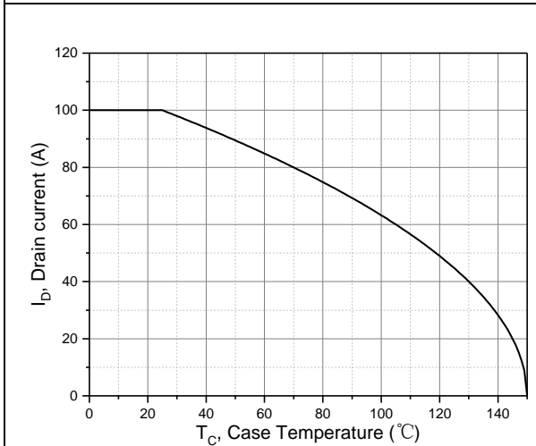
Figure 9. Drain current
